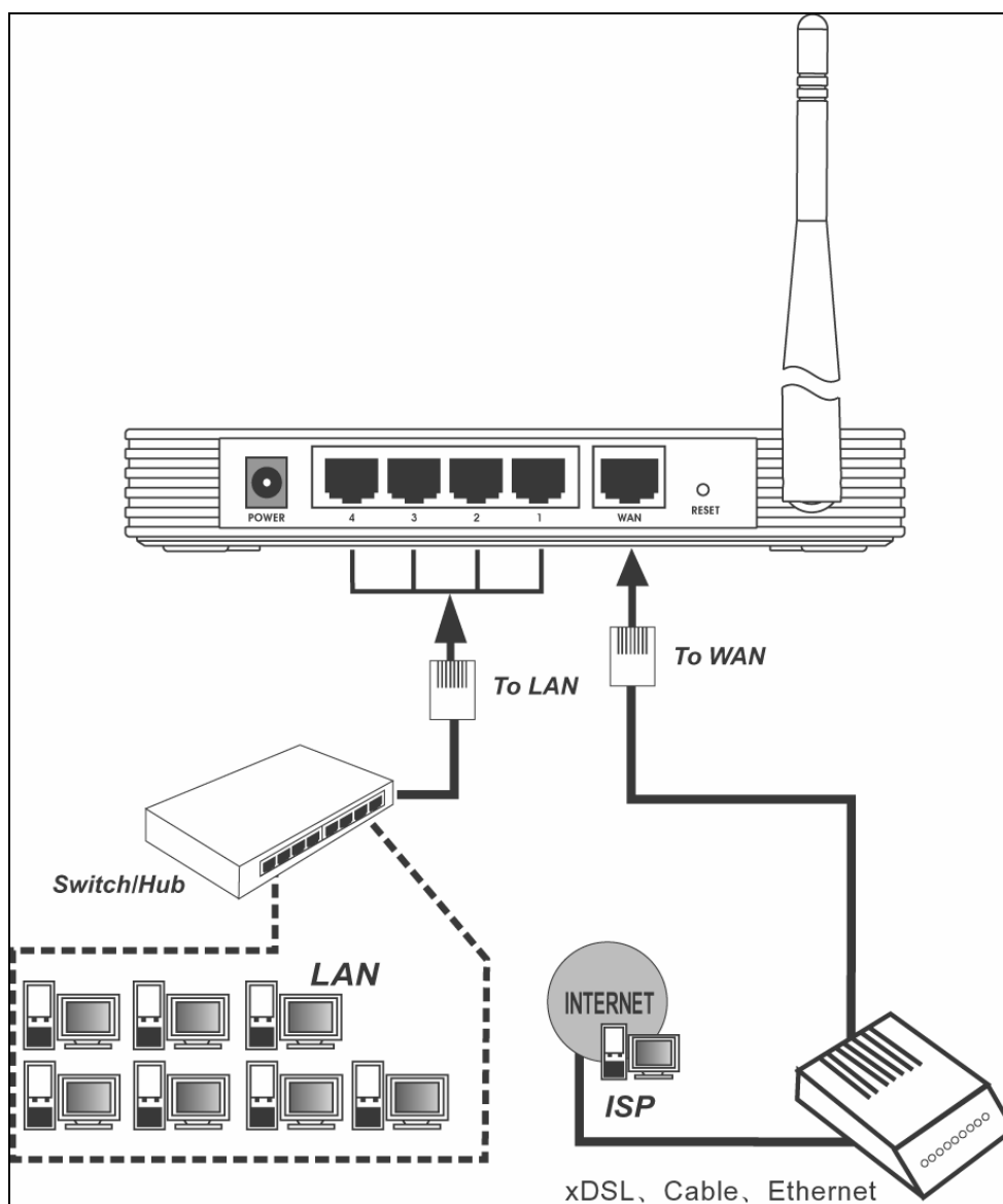
Figure 3-1 Hardware Installation of the TL-WR541G 54Mbps Wireless Router
